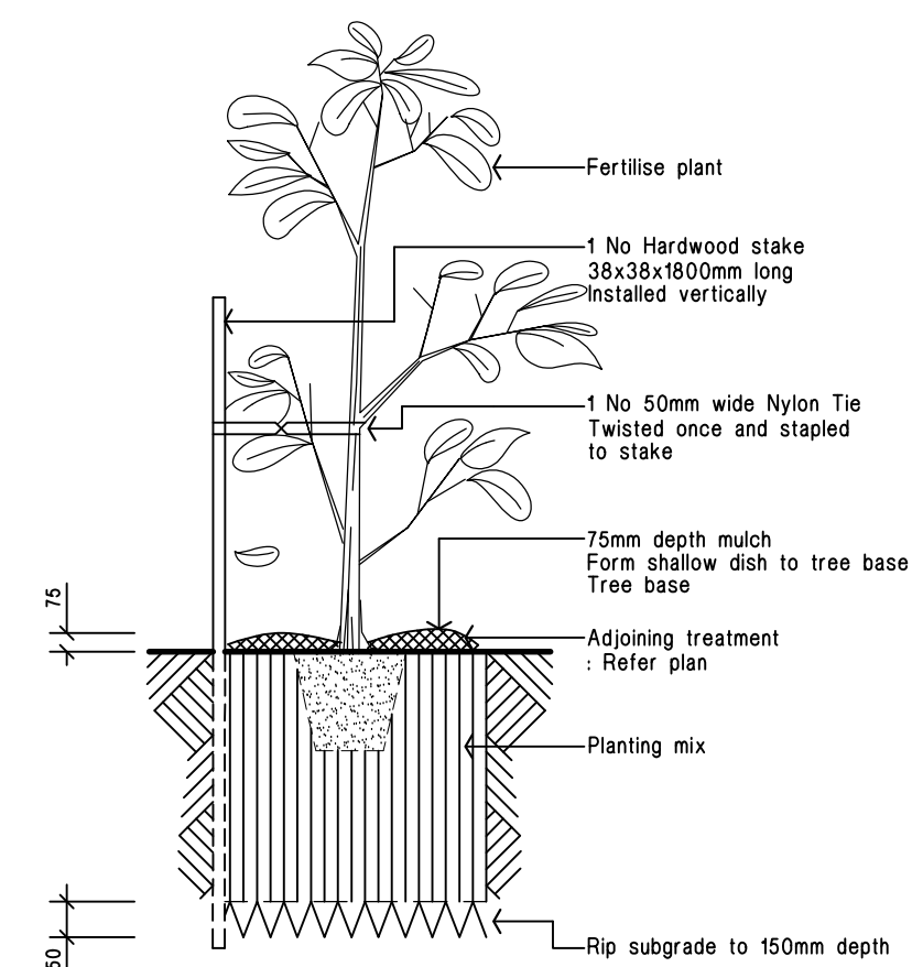
15 - 35 litre Tree planting Detail. Not To Scale.
