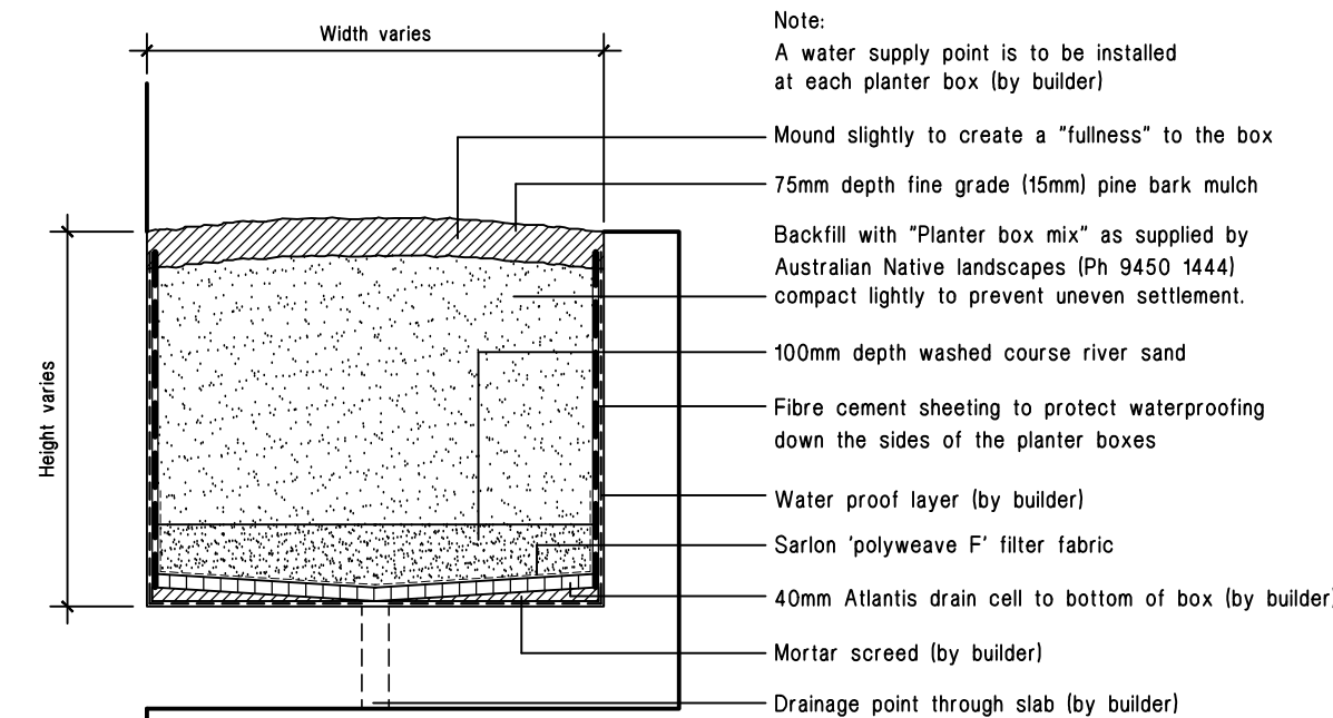
Typical planter box Detail. Not To Scale.
